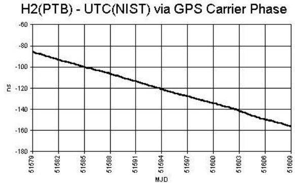
Figure 6 – Comparison between PTB and NIST Frequency Standards using the GPS Carrier-Phase technique
