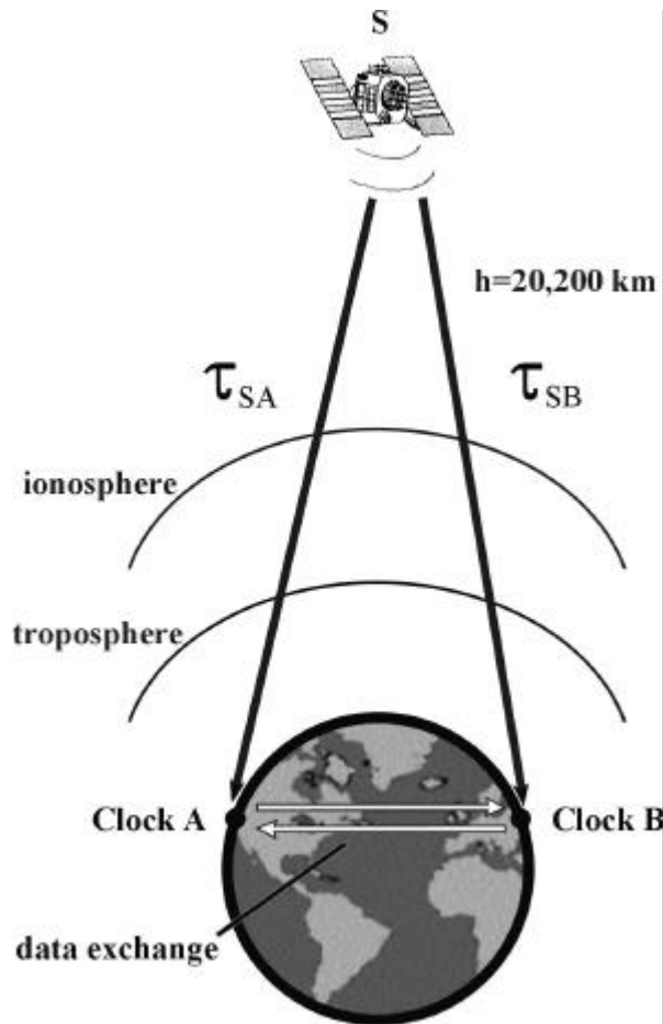
Figure 4 – The common-view measurement technique
