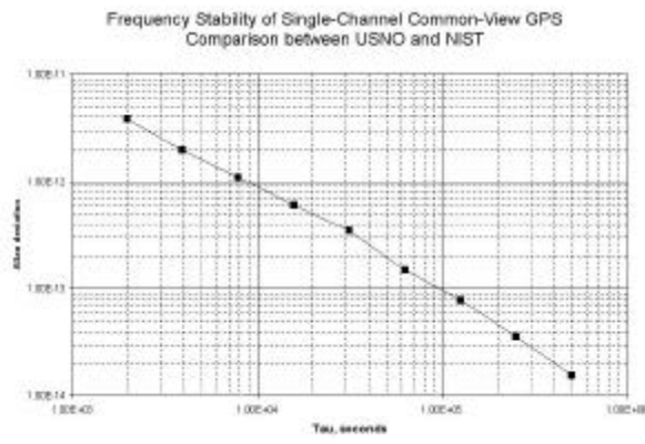
Figure 5 – Frequency stability (Allan deviation) of single-channel common-view comparison between USNO and NIST
