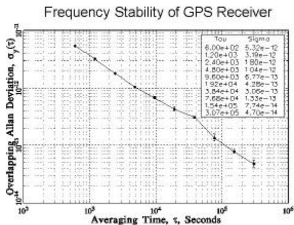
Figure 3 – Frequency stability (Allan deviation) of GPS receiver after SA was set to 0
