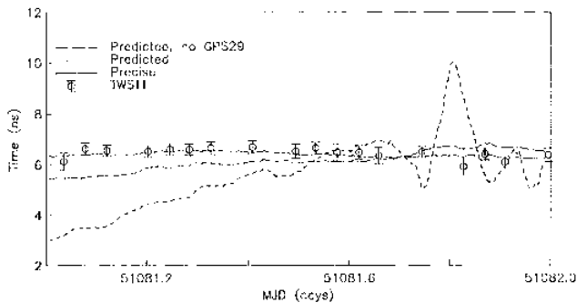
Fig. 12. Carrier-phase clock estimates using precise orbits, predicted orbits (with and without GPS 29), and TWSTT for MJD 51081. TWSTT measurements are shown with error bars indicating 1 standard deviation.
