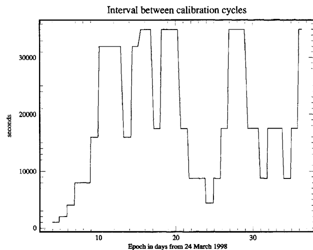
Fig. 2. The interval in seconds between calibration cycles as a function of epoch for the first experiment.
