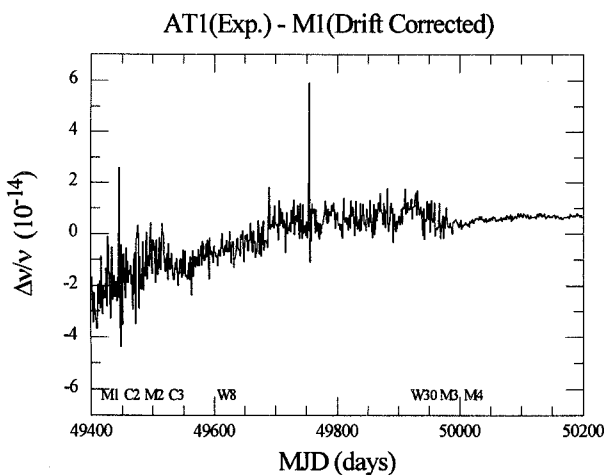
Figure 9 Normalized frequency difference between an experimental AT1 and M1.
