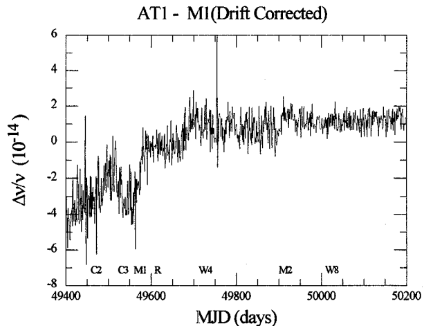
Figure 6 Normalized frequency difference between AT1 and M1.
