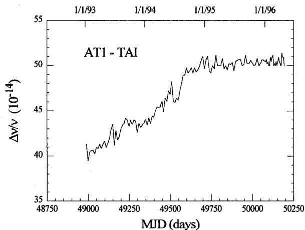
Figure 5 Normalized frequency difference between the NIST AT1 and TAI.
