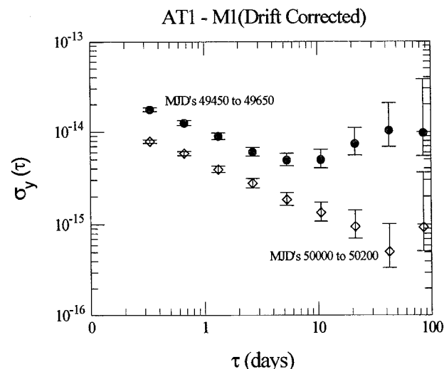
Figure 7 Allan deviation for the data in Fig. 6. Solid circles are from an early 200 day period and the diamonds are for the last 200 days. The error bars are 3\sigma .
