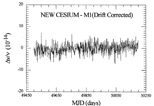
Figure 3 Normalized frequency difference between a new generation high performance cesium standard and maser M1.
