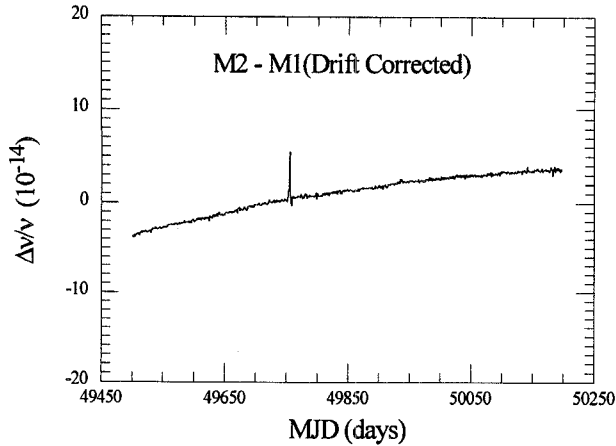
Figure 4 Normalized frequency difference between masers M2 and M1.
