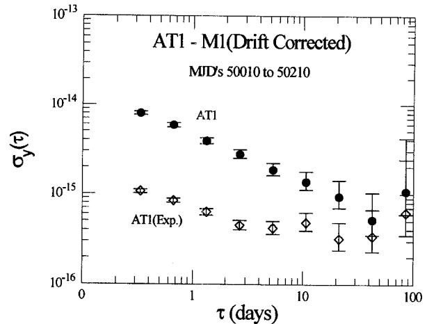
Figure 10 Allan deviation for a recent 200 day period from the real time AT1 (solid circles) and the experimental version of AT1 (diamonds). The error bars are 3\sigma .
