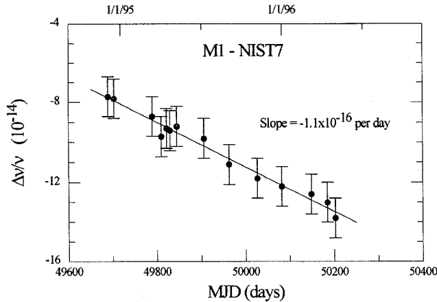
Figure 1 Normalized frequency difference between maser M1 and NIST-7.
