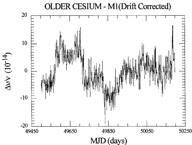
Figure 2 Normalized frequency difference between an older generation high performance cesium standard and maser M1.
