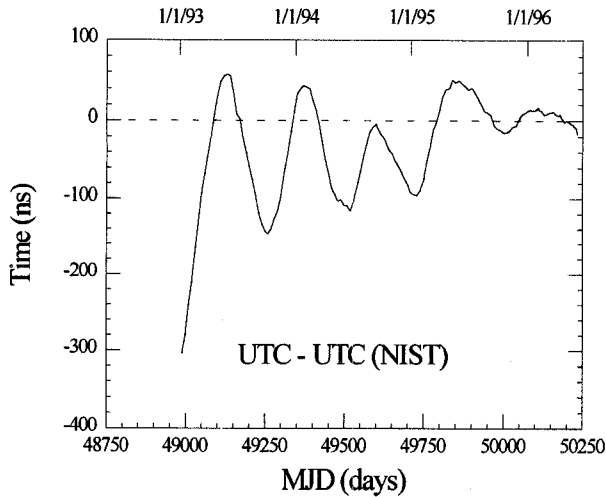
Figure 8 Difference between UTC and UTC(NIST).
