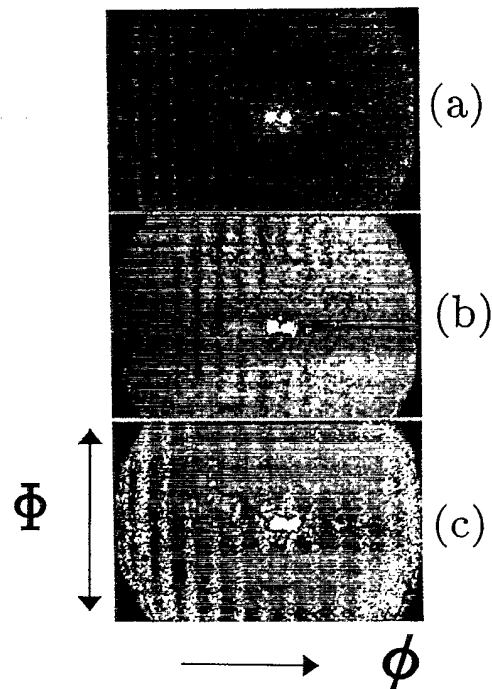
FIG. 2. Interference pattern for three different ion separations: (a) 5.4 \mu\text{m} , (b) 4.3 \mu\text{m} , and (c) 3.7 \mu\text{m} . The two white spots are caused by stray reflections of the laser beam.
